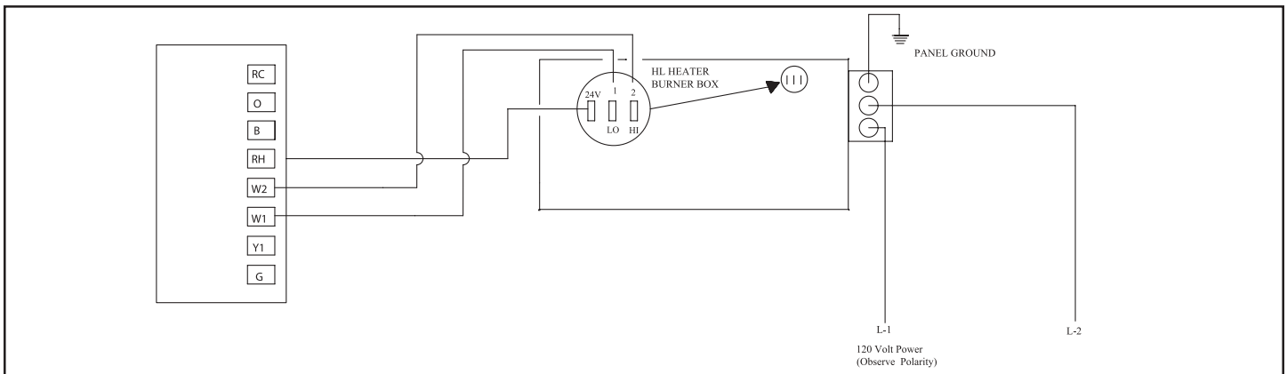
Two-stage heaters with a PSP-602 thermostat. Single heater, single thermostat. No HLRB (relay board) is installed.
